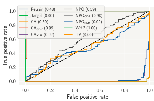
Figure 4: ROC curves for \mathcal{D}_{\text{forget}} vs. \mathcal{D}_{\text{holdout}} on NEWS using Min-K% Prob, with AUC scores in parentheses. \text{AUC} \approx 0.5 (i.e., f_{\text{retrained}} ) means no significant distribution difference between two sets (i.e., no membership leakage). Most unlearning methods show under-unlearn ( \text{AUC} \ll 0.5 ) or over-unlearn ( \text{AUC} \gg 0.5 ).
